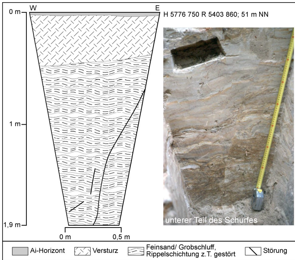
Abb. 86: Schurf Neu2
