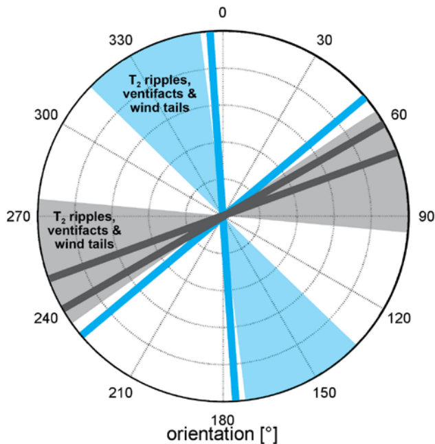
Fig. 40 - Rose diagram summarising wind directions in the Columbia Hills. Sectors with solid colours are wind directions inferred from ventifacts, wind tails and 2nd-order bedforms (T 2 ) from photographic interpretation of these aeolian features by Greeley et al. (2008) and Thomson et al. (2008). Solid lines are the preferred orientations of particles measured in the sediment fabric of the three surface targets in this study. Blue sectors and lines correspond to El Dorado; those in grey give the headings for Home Plate.
